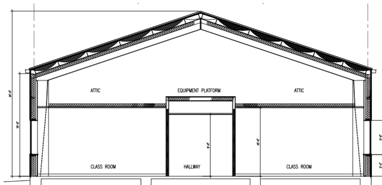
02 BUILDING SECTION AT CLASSROOMS 3/8" = 1'-0"
