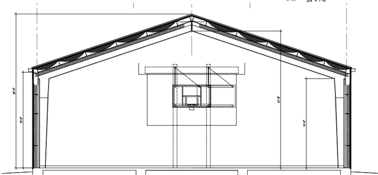
01 BUILDING SECTION AT GYM (50'x125') 3/8" = 1'-0"
